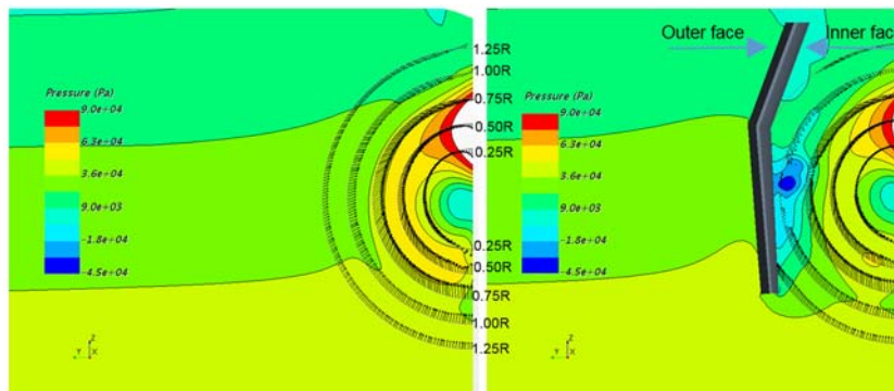
Figure 13. CFD arrangement of gate rudders with actuator disc as a representative propeller
