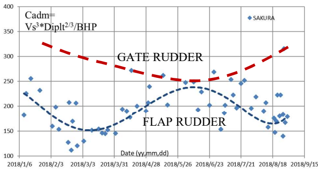
Figure 7. Trend of Admiralty coefficients based on logbook data of two sister ships (Jan. –Sept.2018)
